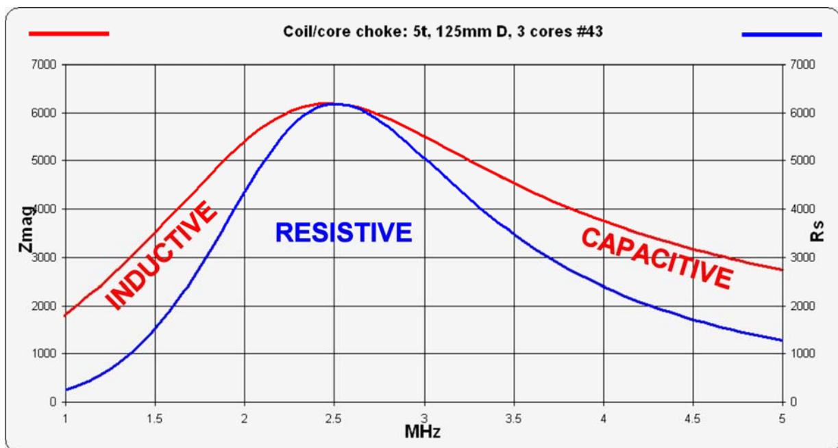
FIGURE 3: Performance of the Low Bands choke with three ferrite cores.
