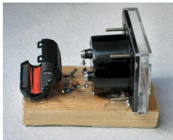
Figure 9: A simple and effective RF current meter.
