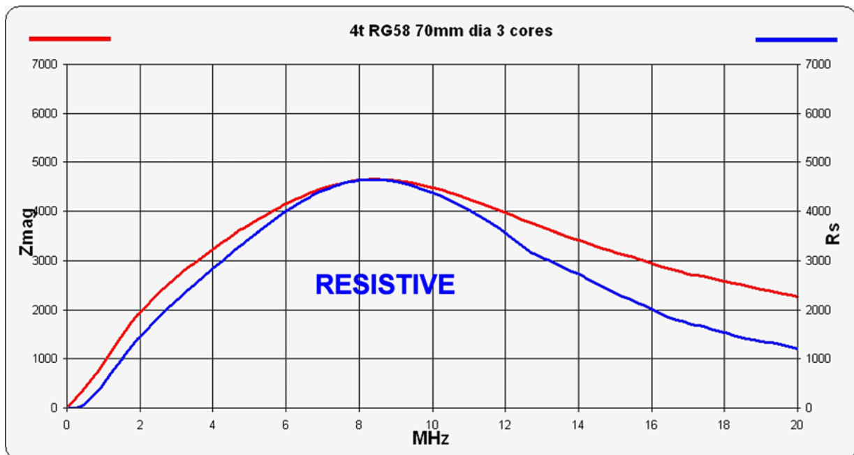
FIGURE 4: Performance of the smaller Mid Bands choke.
